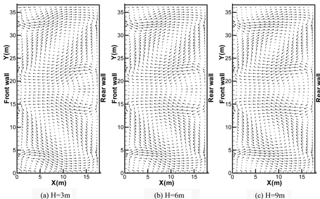
Fig. 7. Cross-sectional velocity distributions in the main burner zone with different OFA positions.
