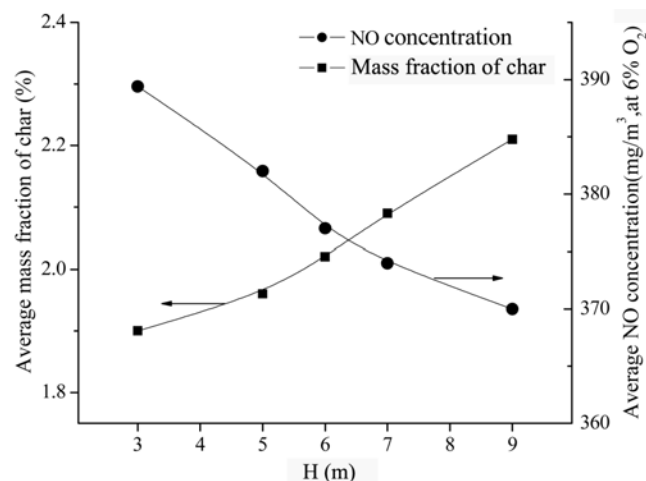
Fig. 9. Average mass fractions of char (%) and average NO concentrations ( \text{mg/m}^3 , at 6% \text{O}_2 ) at the outlet in five scenarios.
